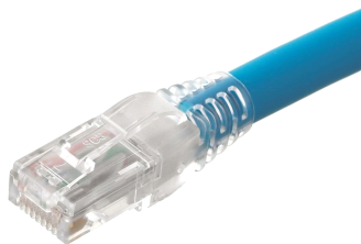
RJ45 Patch Cord, category 6, 8-position, plug to plug, unshielded, blue, 10 ft
