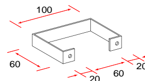
"C" Support
